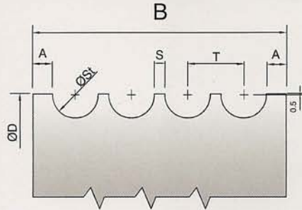
Round Rod Milling Cutter
